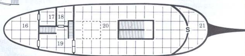
Cargo Deck
